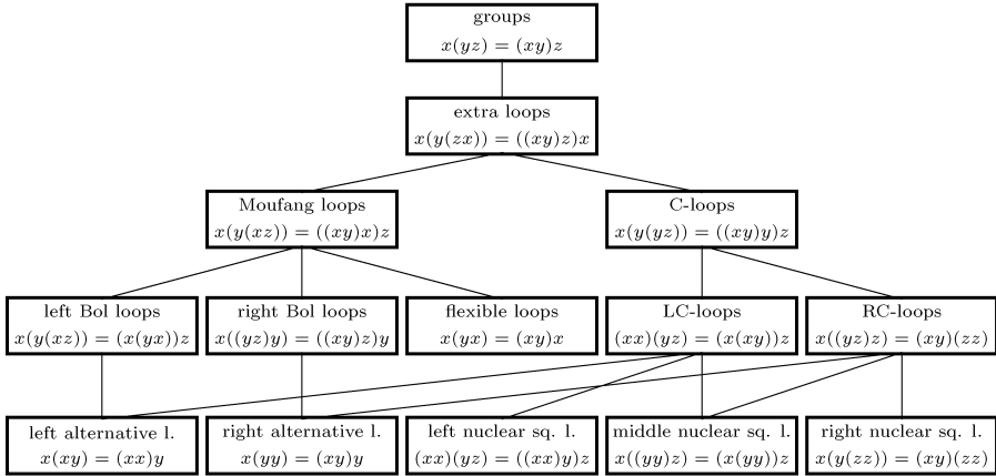
FIGURE 2. The varieties of loops of Bol-Moufang type
