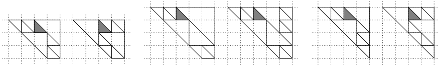
FIGURE 7. Proper triangulations for Subcase B of Lemma 4.1.
