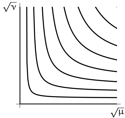
FIGURE 2. FS of the Neumann problem
